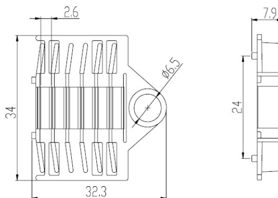
Mechanical Diagram
