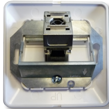
rear view ET-25108 assembled
